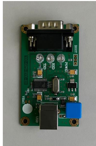
Adaptor Board
