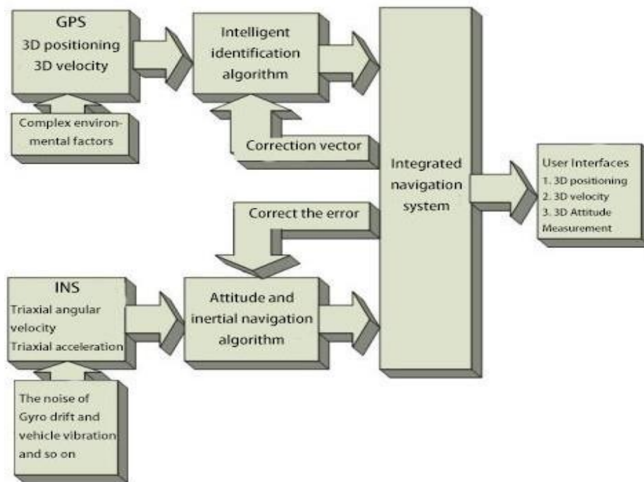
Figure 1-2 : Block Diagram
